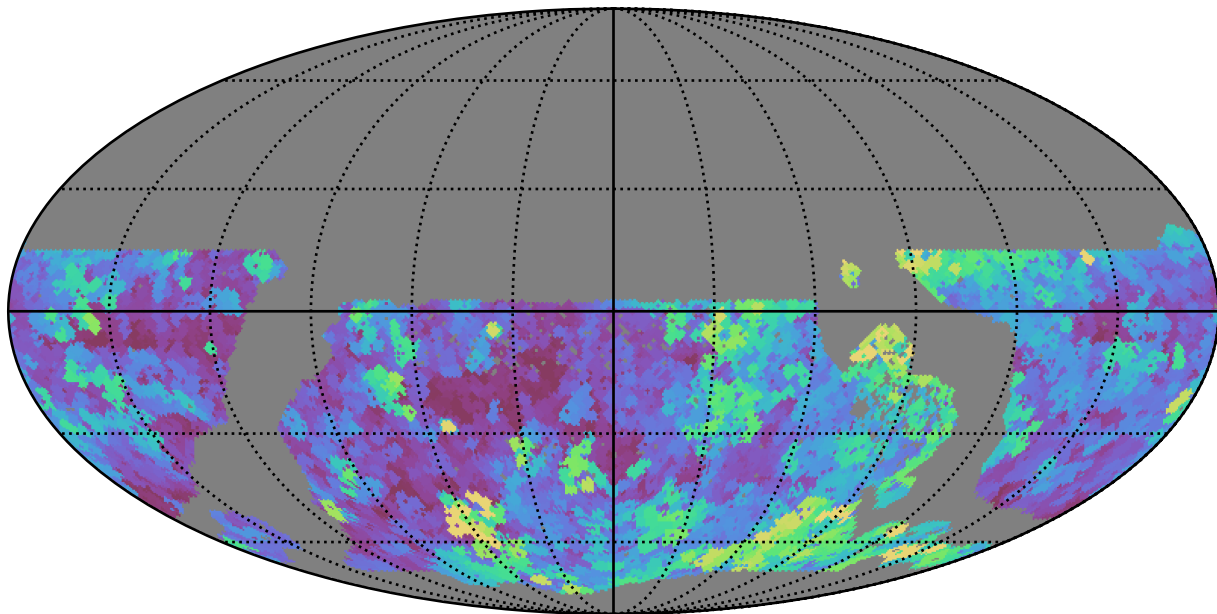
no_magell_roll_v3.4_10yrs WFD g band: Max seeingEff
