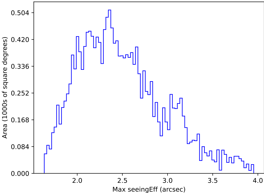
no_magell_roll_v3.4_10yrs WFD g band: Max seeingEff
