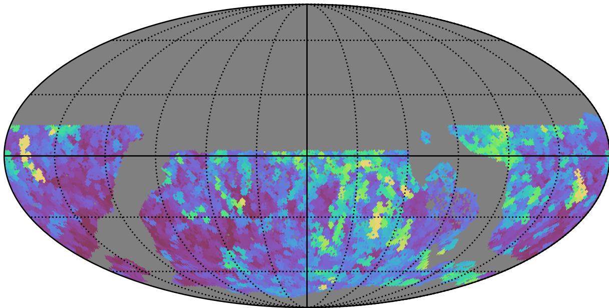
no_magell_roll_v3.4_10yrs WFD all bands: Max seeingEff
