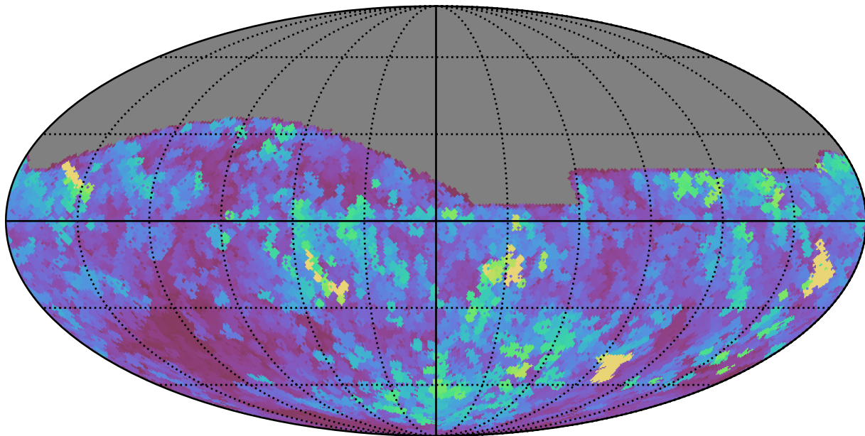
no_magell_roll_v3.4_10yrs All sky z band: Max seeingEff
