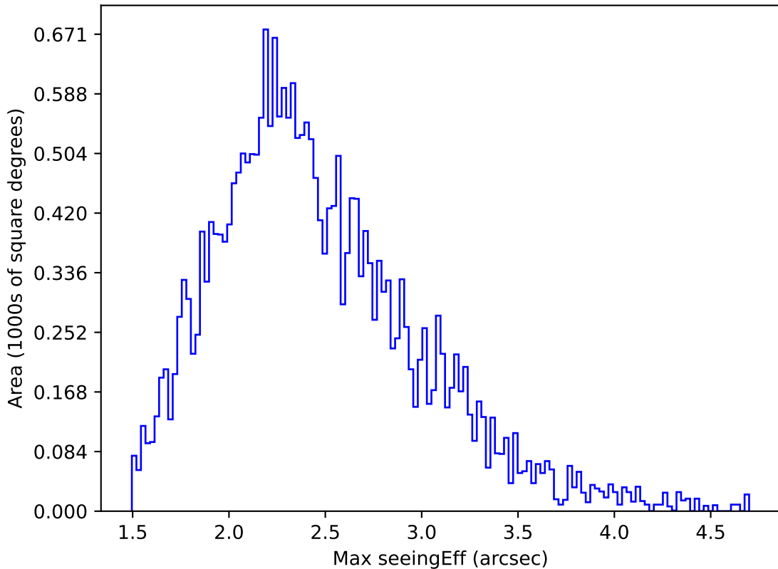
no_magell_roll_v3.4_10yrs All sky z band: Max seeingEff
