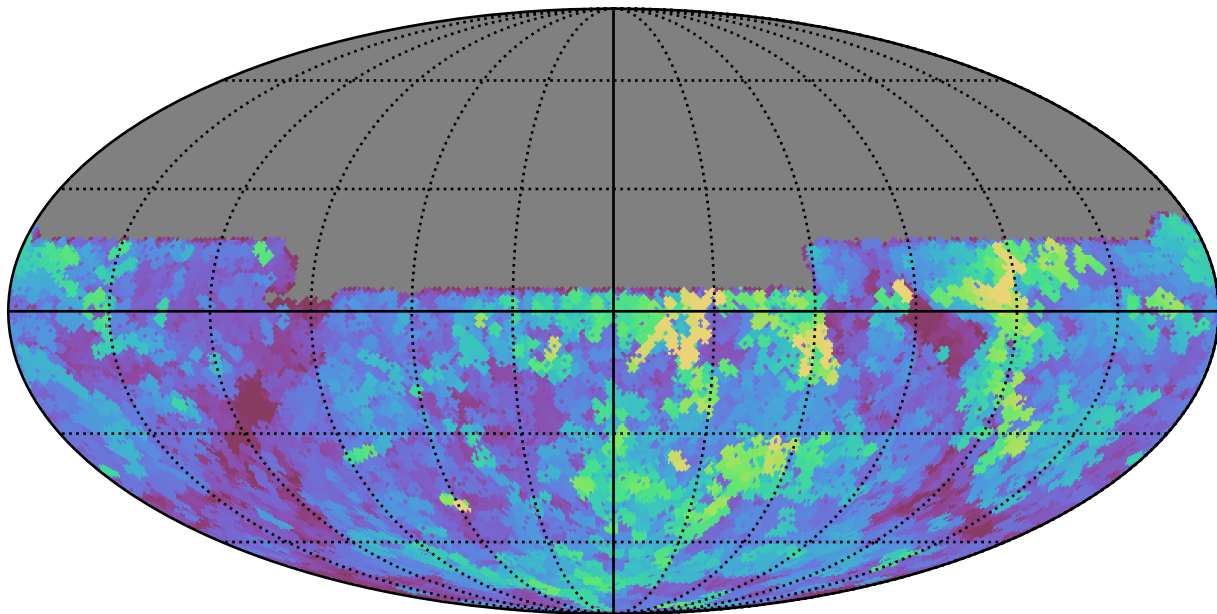
no_magell_roll_v3.4_10yrs All sky u band: Max seeingEff
