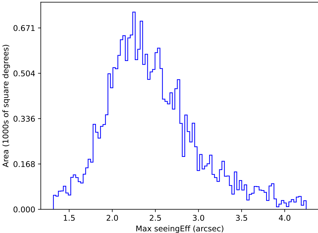
no_magell_roll_v3.4_10yrs All sky u band: Max seeingEff
