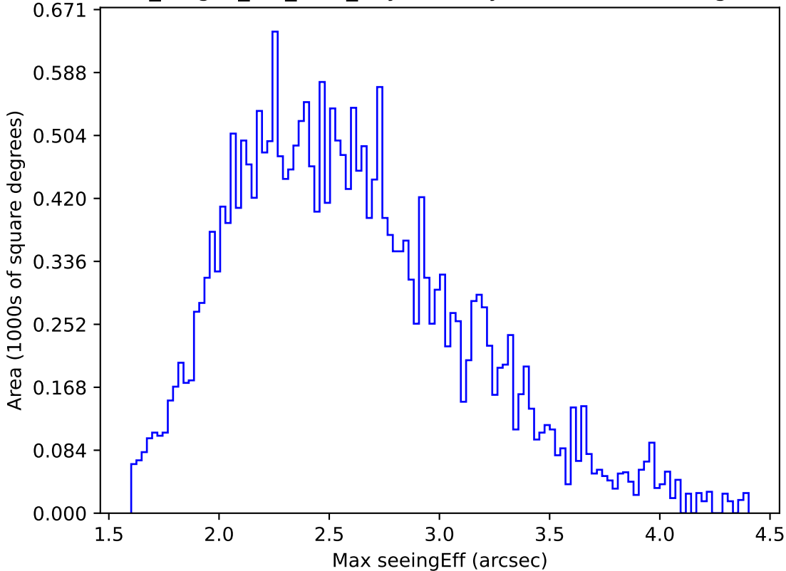
no_magell_roll_v3.4_10yrs All sky r band: Max seeingEff
