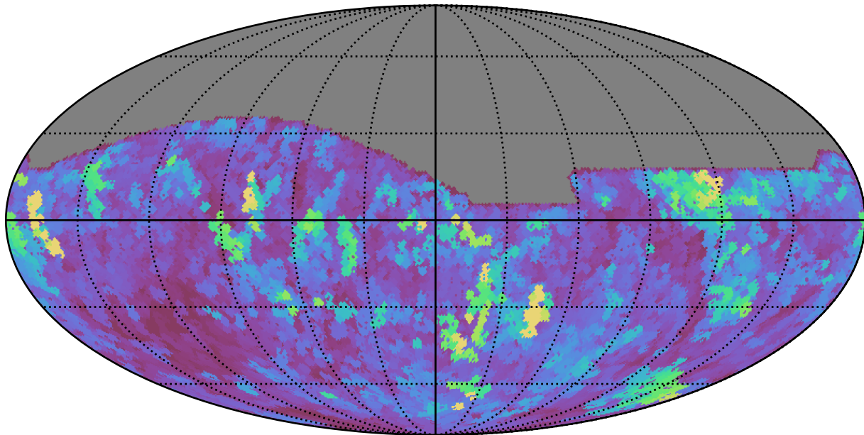
no_magell_roll_v3.4_10yrs All sky i band: Max seeingEff
