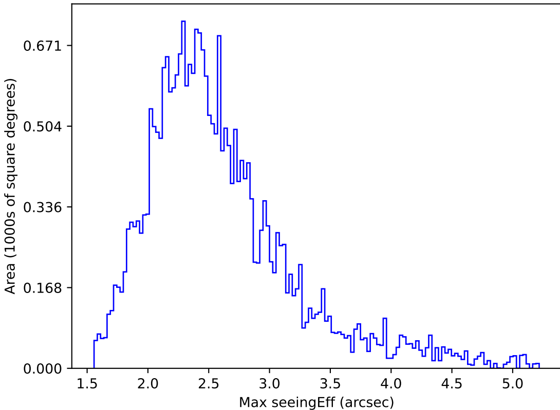
no_magell_roll_v3.4_10yrs All sky i band: Max seeingEff
