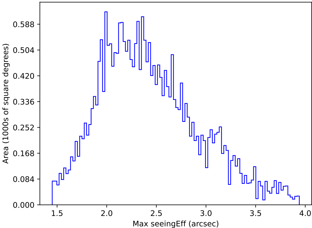
no_magell_roll_v3.4_10yrs All sky g band: Max seeingEff
