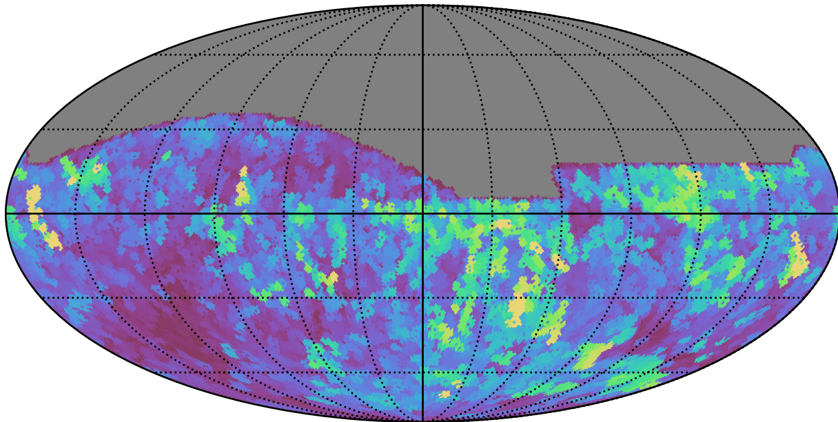
no_magell_roll_v3.4_10yrs All sky all bands: Max seeingEff
