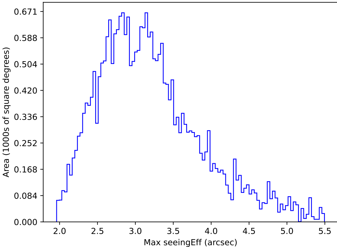
no_magell_roll_v3.4_10yrs All sky all bands: Max seeingEff
