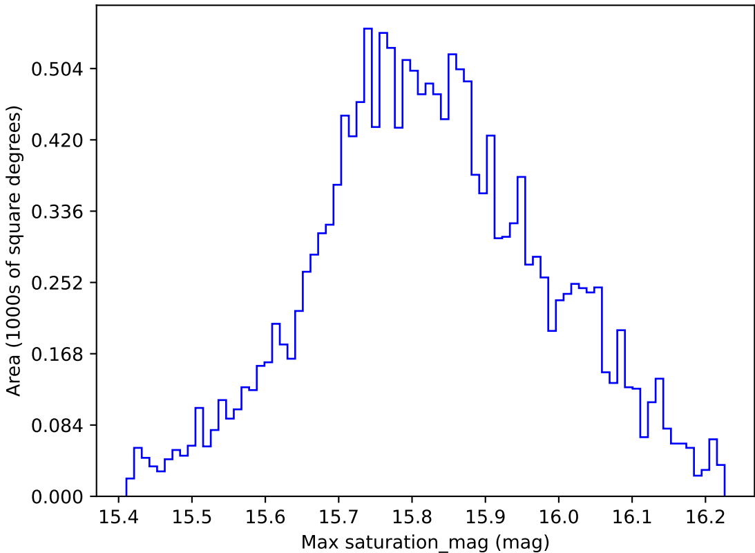
no_magell_roll_v3.4_10yrs WFD all bands: Max saturation_mag
