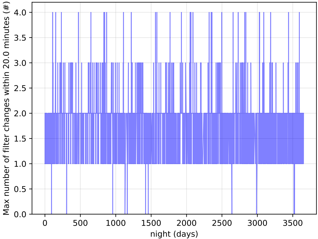
no_magell_roll_v3.4_10yrs Per Night: Max number of filter changes within 20.0 minutes
