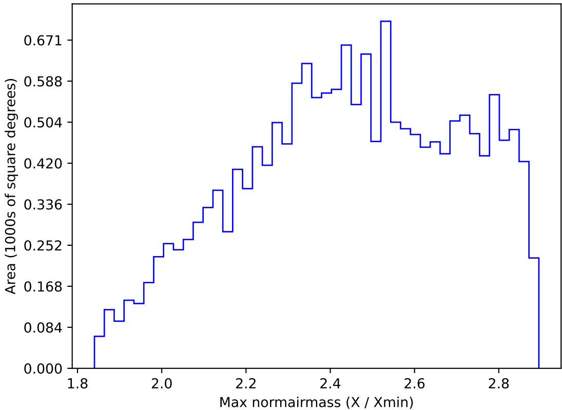
no_magell_roll_v3.4_10yrs WFD all bands: Max normairmass
