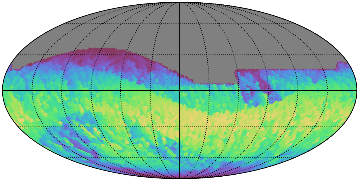
no_magell_roll_v3.4_10yrs All sky all bands: Max normairmass
