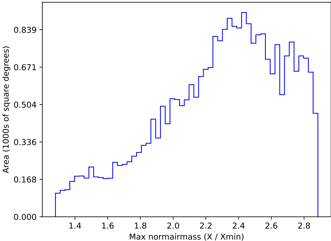
no_magell_roll_v3.4_10yrs All sky all bands: Max normairmass
