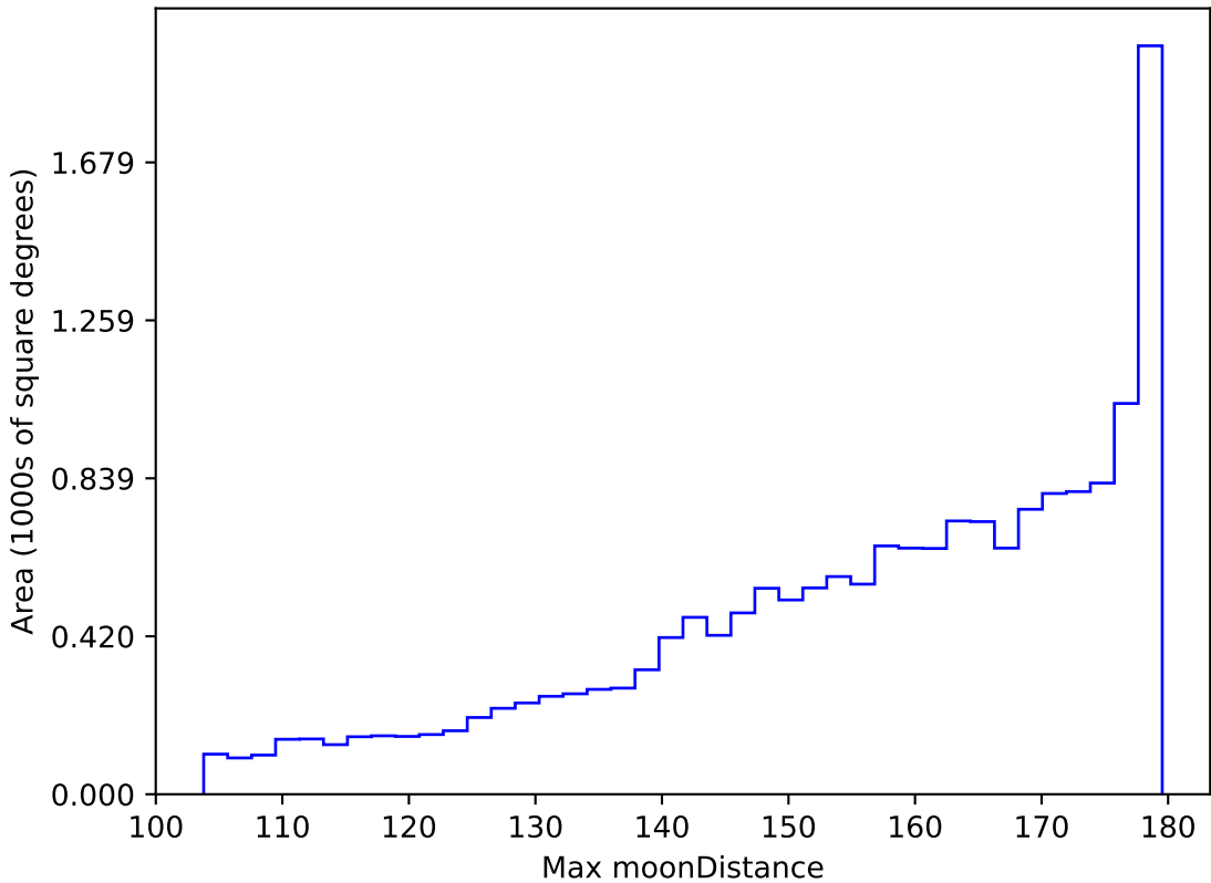
no_magell_roll_v3.4_10yrs WFD all bands: Max moonDistance
