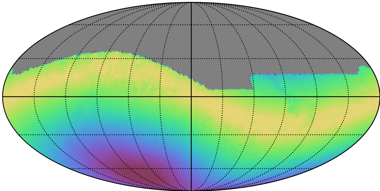
no_magell_roll_v3.4_10yrs All sky all bands: Max moonDistance
