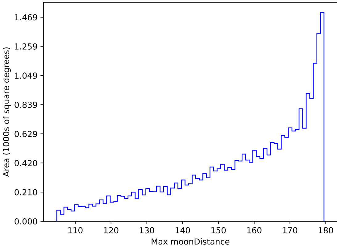
no_magell_roll_v3.4_10yrs All sky all bands: Max moonDistance
