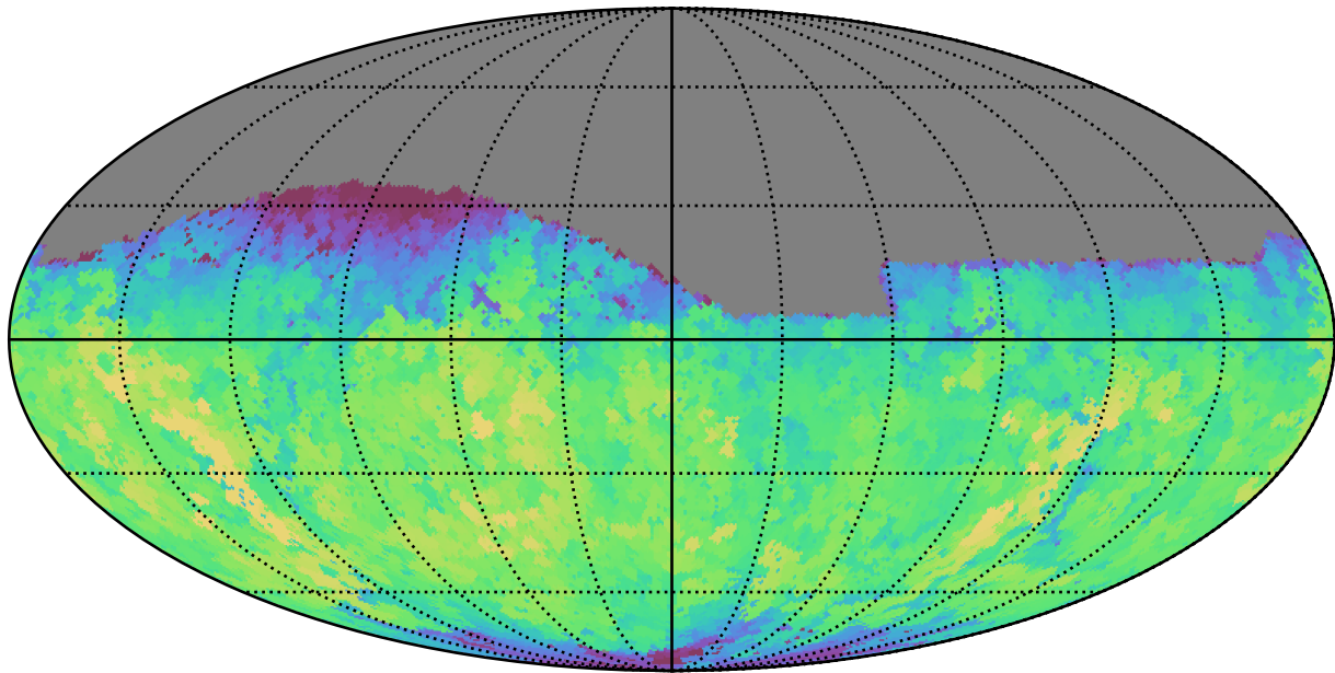
no_magell_roll_v3.4_10yrs Yr 1 z band: Max fiveSigmaDepth
