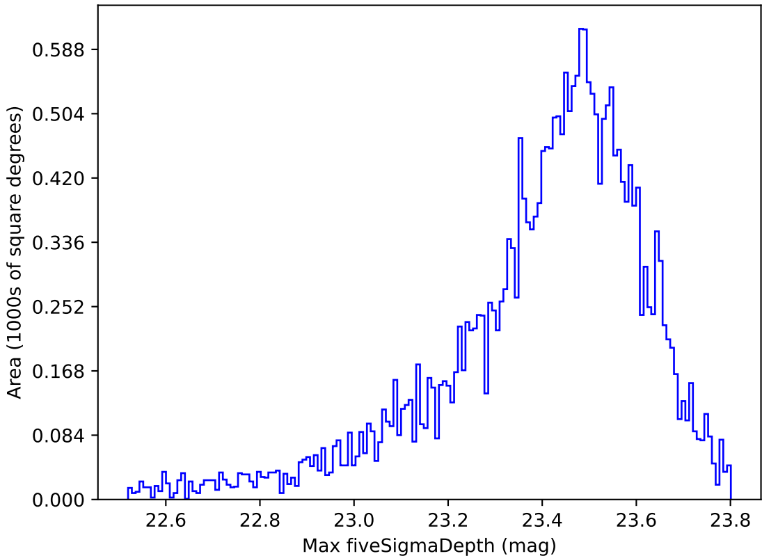
no_magell_roll_v3.4_10yrs Yr 1 z band: Max fiveSigmaDepth
