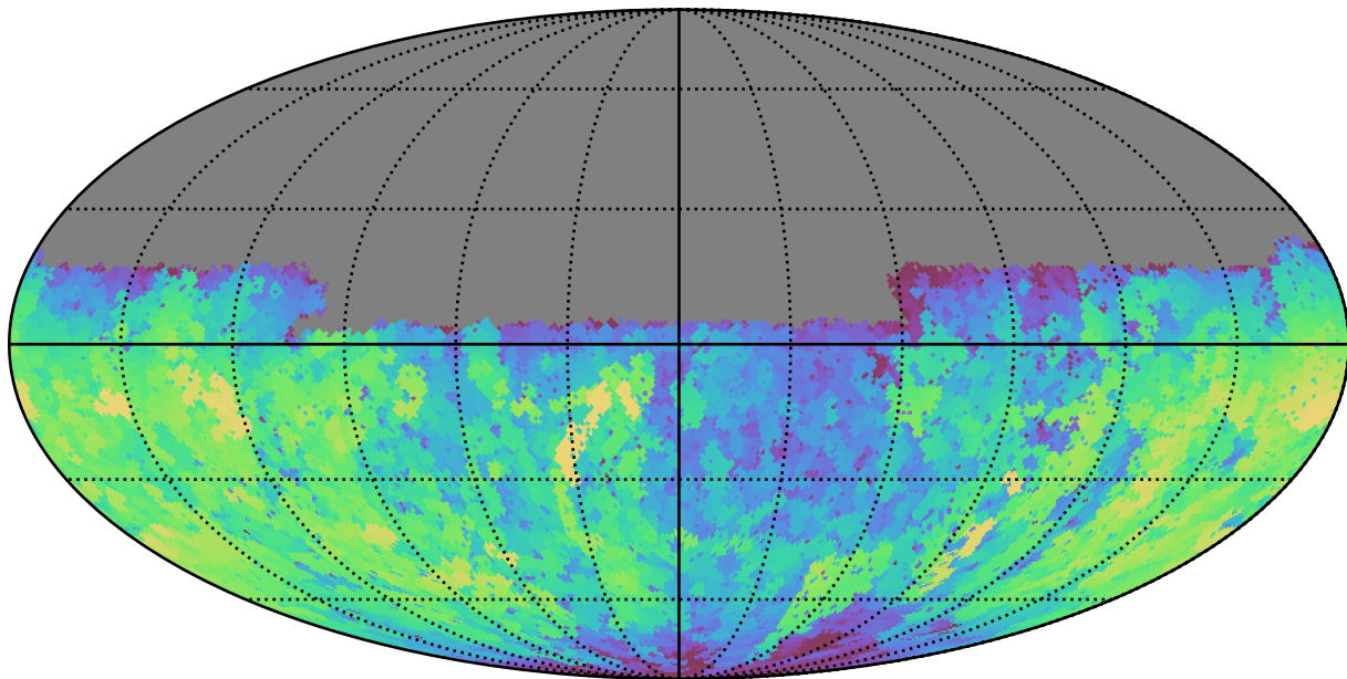
no_magell_roll_v3.4_10yrs Yr 1 u band: Max fiveSigmaDepth
