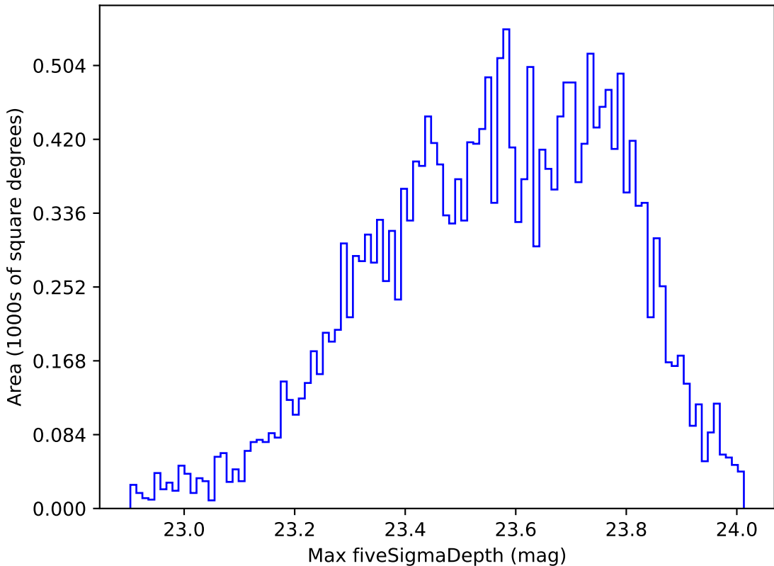
no_magell_roll_v3.4_10yrs Yr 1 u band: Max fiveSigmaDepth
