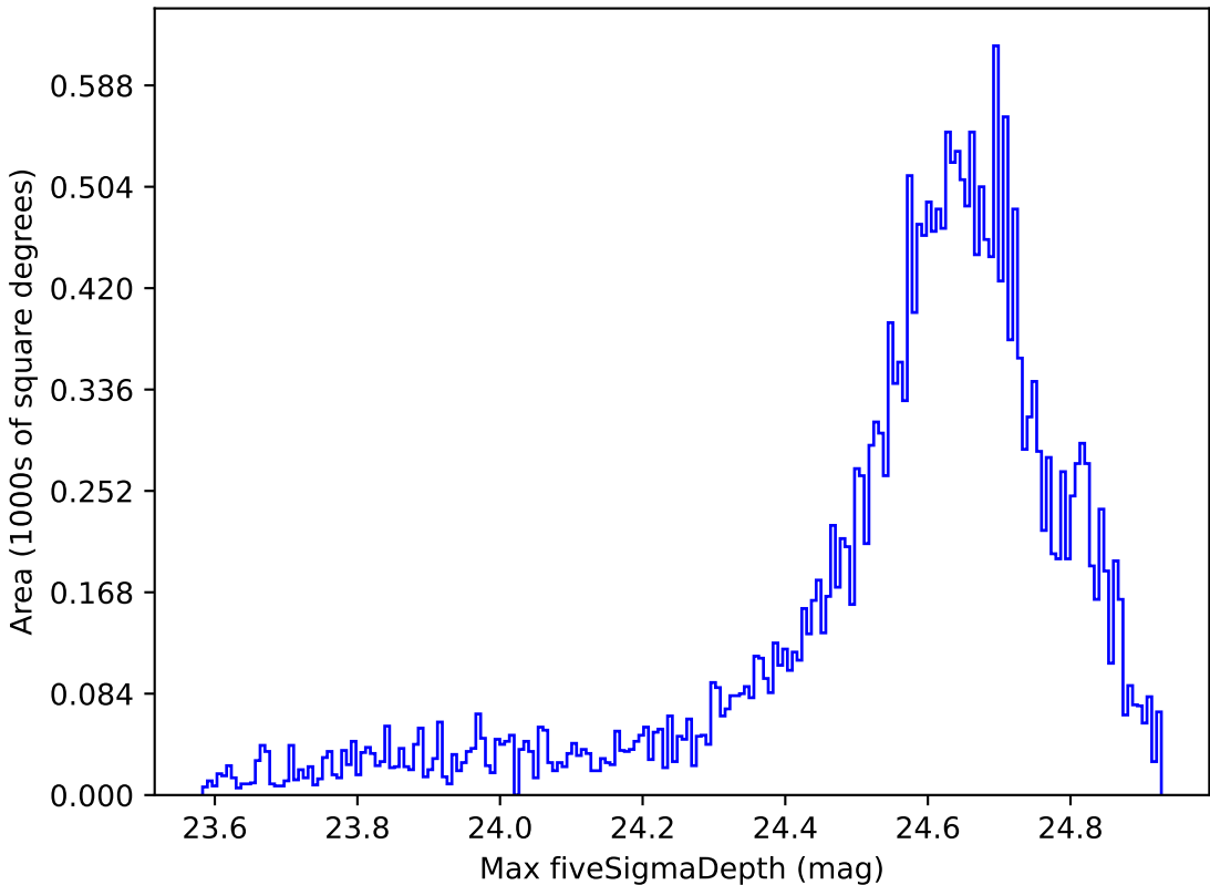
no_magell_roll_v3.4_10yrs Yr 1 r band: Max fiveSigmaDepth
