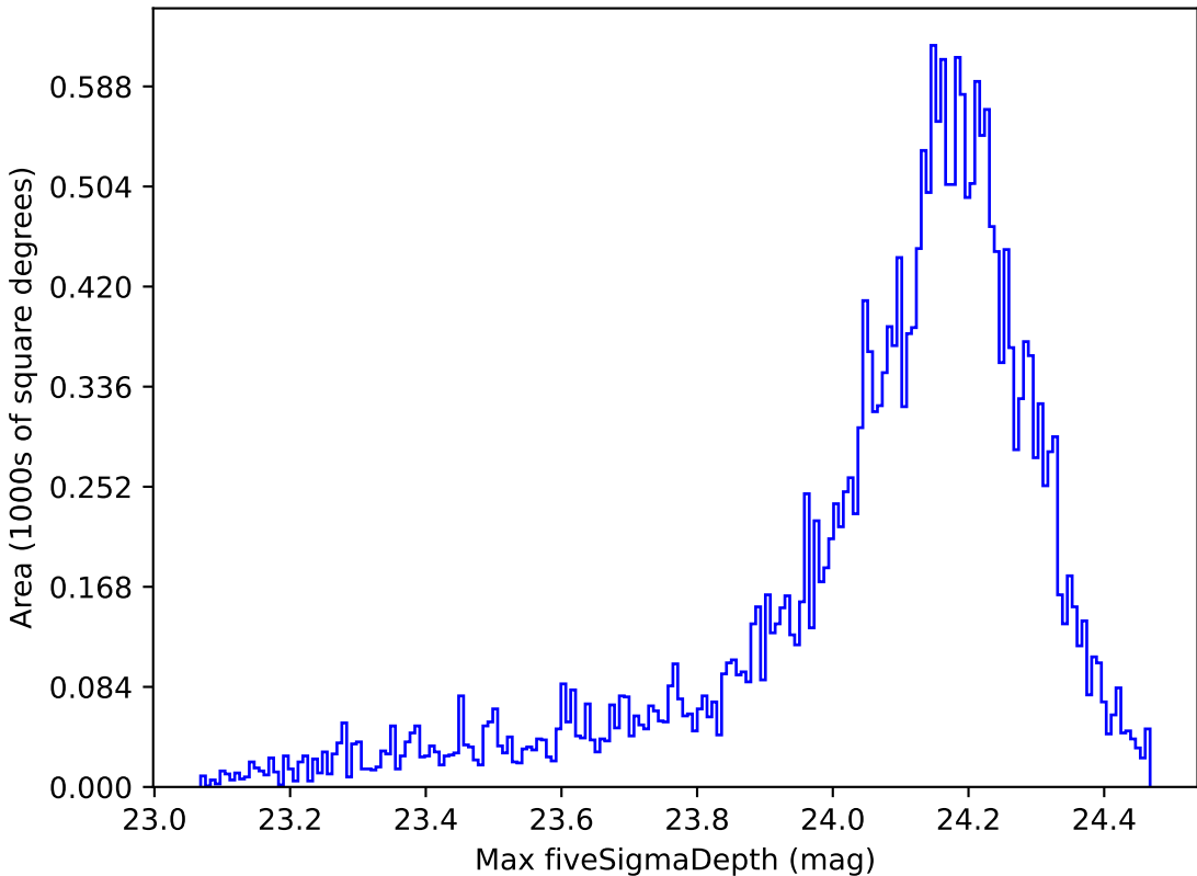
no_magell_roll_v3.4_10yrs Yr 1 i band: Max fiveSigmaDepth
