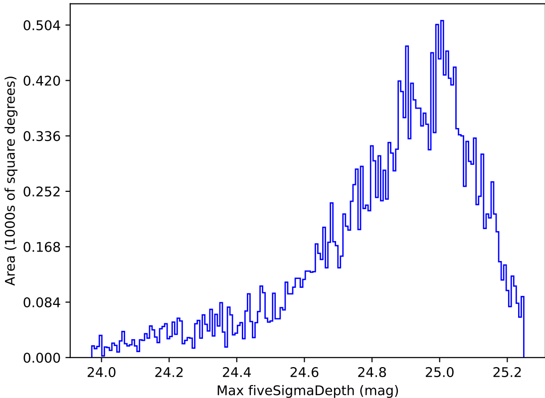
no_magell_roll_v3.4_10yrs Yr 1 g band: Max fiveSigmaDepth
