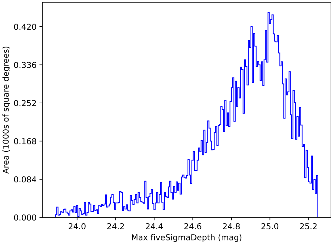
no_magell_roll_v3.4_10yrs Yr 1 all bands: Max fiveSigmaDepth
