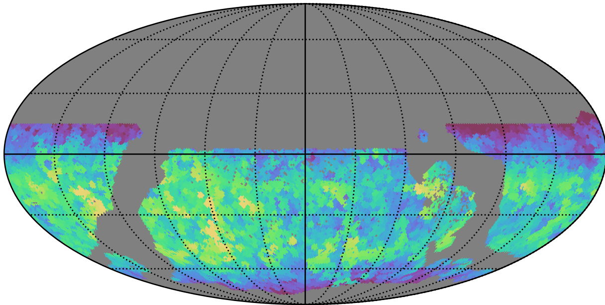
no_magell_roll_v3.4_10yrs WFD z band: Max fiveSigmaDepth
