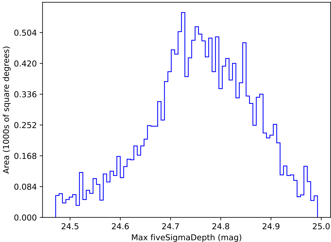
no_magell_roll_v3.4_10yrs WFD r band: Max fiveSigmaDepth
