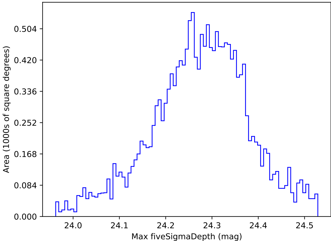
no_magell_roll_v3.4_10yrs WFD i band: Max fiveSigmaDepth
