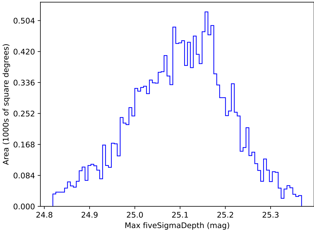
no_magell_roll_v3.4_10yrs WFD g band: Max fiveSigmaDepth
