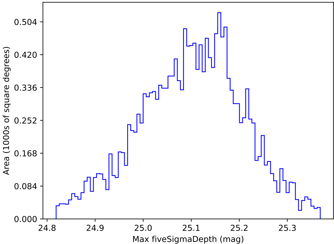
no_magell_roll_v3.4_10yrs WFD all bands: Max fiveSigmaDepth
