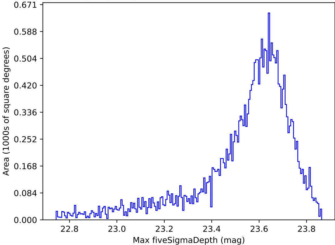
no_magell_roll_v3.4_10yrs All sky z band: Max fiveSigmaDepth
