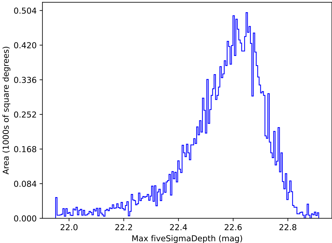
no_magell_roll_v3.4_10yrs All sky y band: Max fiveSigmaDepth
