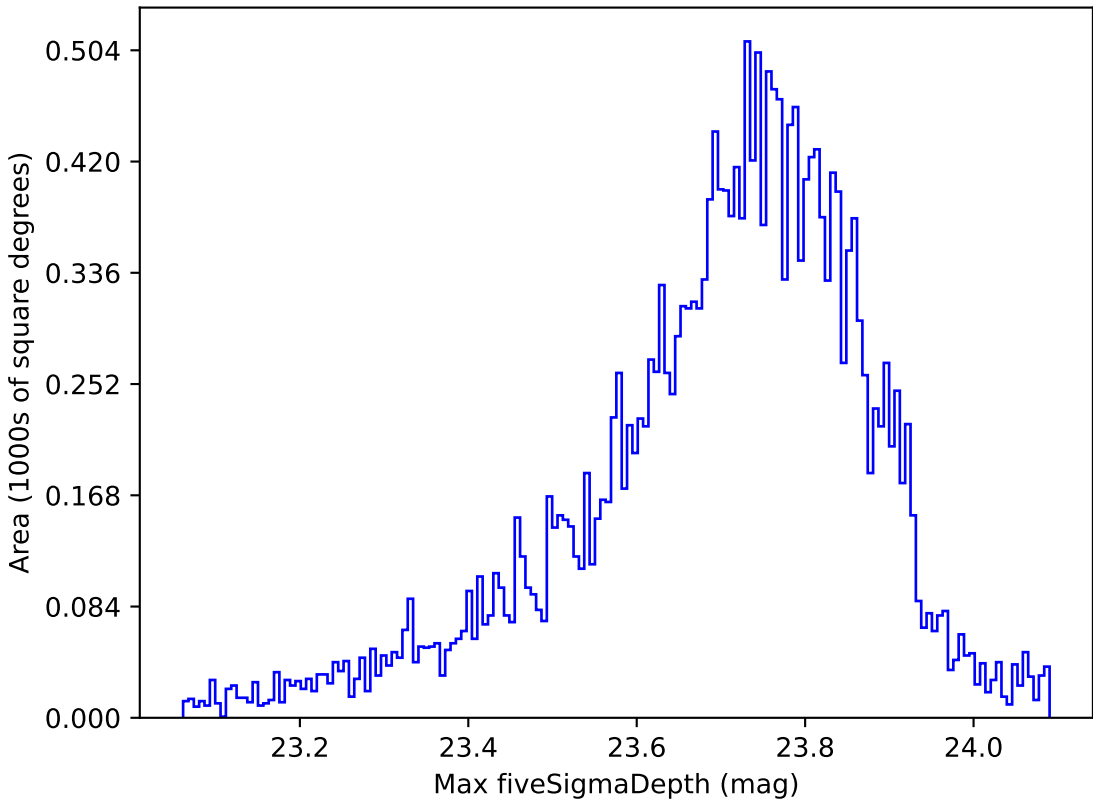
no_magell_roll_v3.4_10yrs All sky u band: Max fiveSigmaDepth
