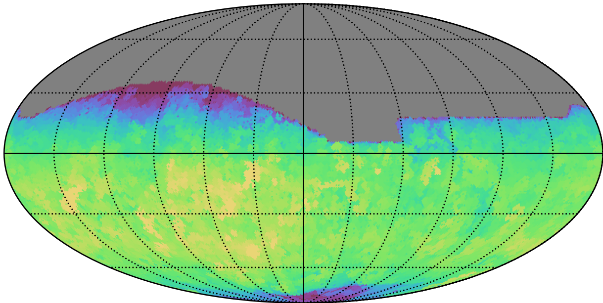
no_magell_roll_v3.4_10yrs All sky r band: Max fiveSigmaDepth
