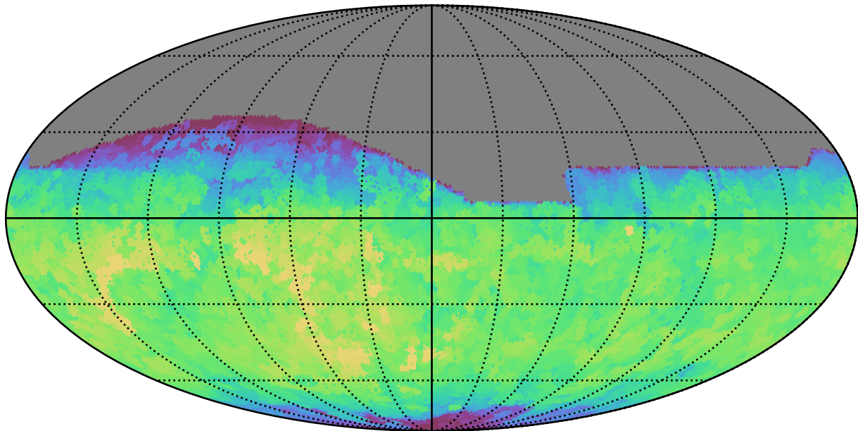
no_magell_roll_v3.4_10yrs All sky i band: Max fiveSigmaDepth
