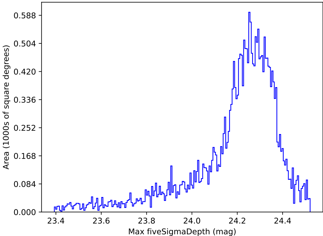
no_magell_roll_v3.4_10yrs All sky i band: Max fiveSigmaDepth
