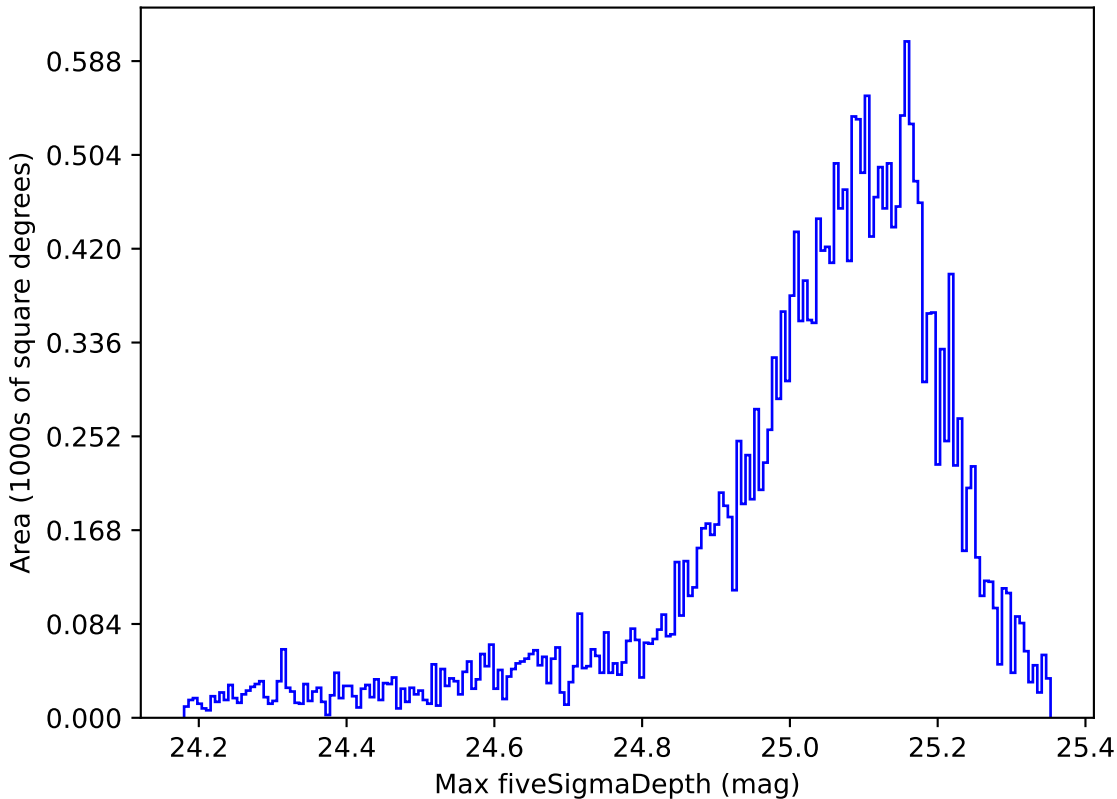
no_magell_roll_v3.4_10yrs All sky g band: Max fiveSigmaDepth
