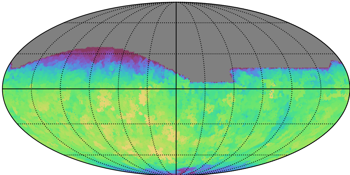
no_magell_roll_v3.4_10yrs All sky all bands: Max fiveSigmaDepth
