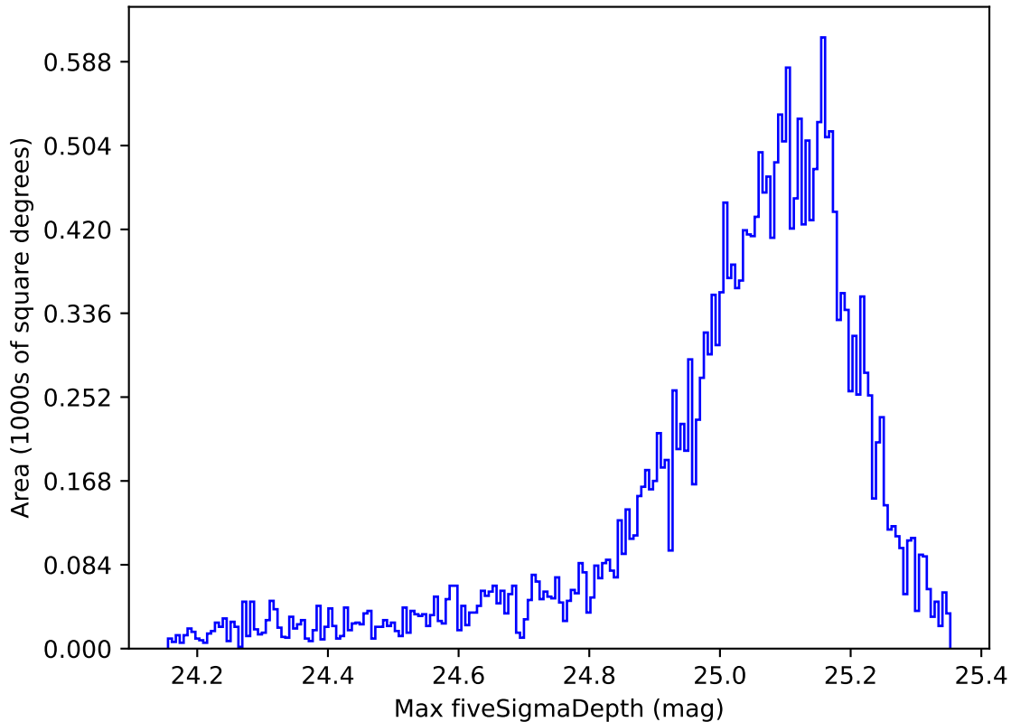
no_magell_roll_v3.4_10yrs All sky all bands: Max fiveSigmaDepth
