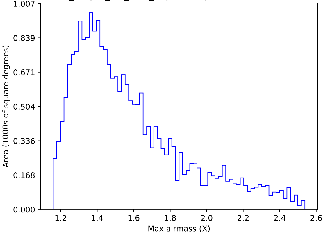
no_magell_roll_v3.4_10yrs Yr 1 y band: Max airmass
