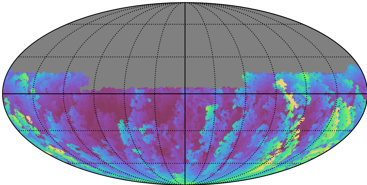
no_magell_roll_v3.4_10yrs Yr 1 u band: Max airmass
