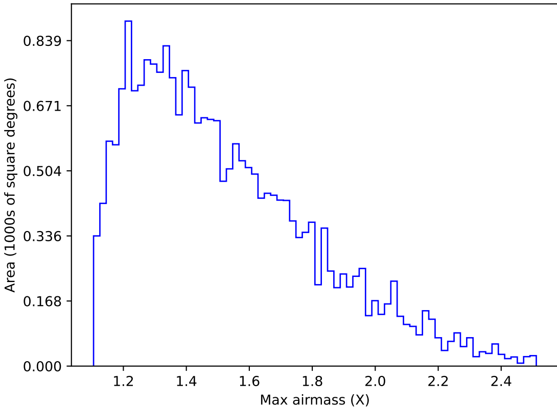
no_magell_roll_v3.4_10yrs Yr 1 u band: Max airmass
