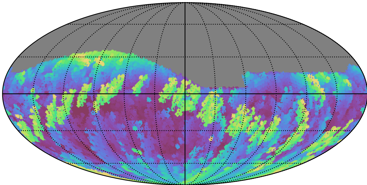
no_magell_roll_v3.4_10yrs Yr 1 r band: Max airmass
