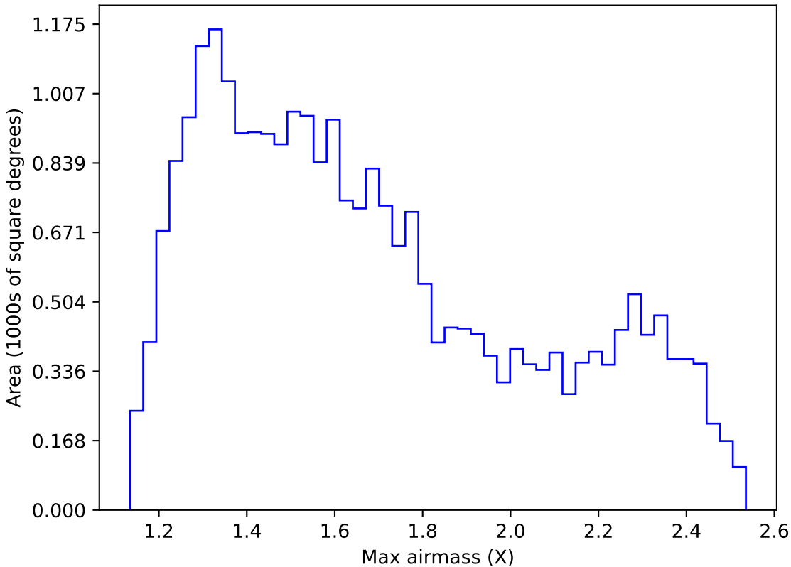
no_magell_roll_v3.4_10yrs Yr 1 r band: Max airmass
