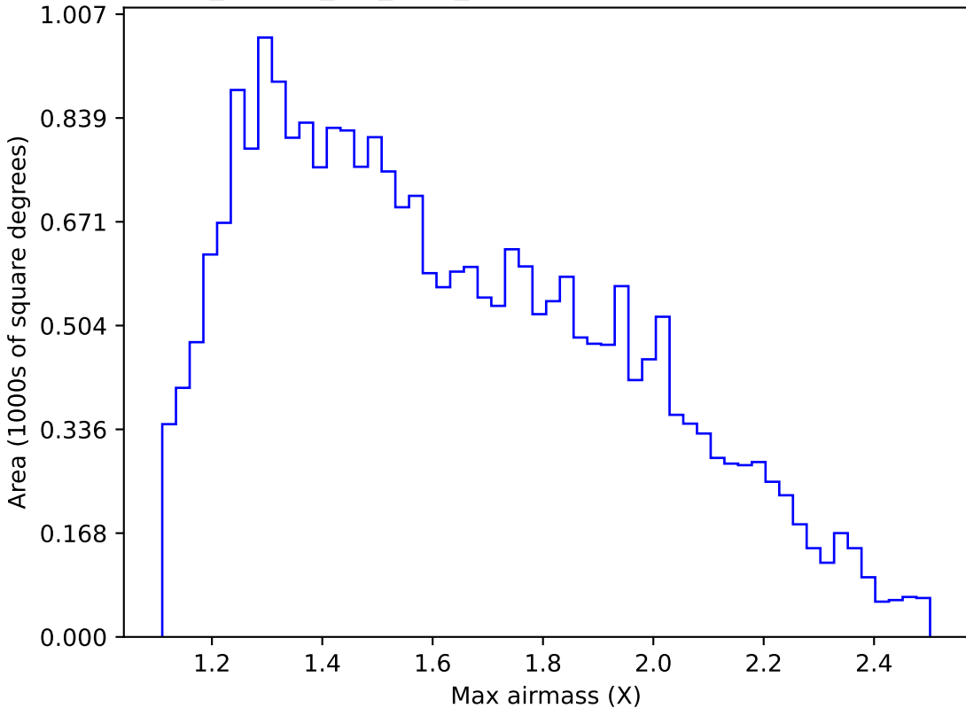
no_magell_roll_v3.4_10yrs Yr 1 g band: Max airmass
