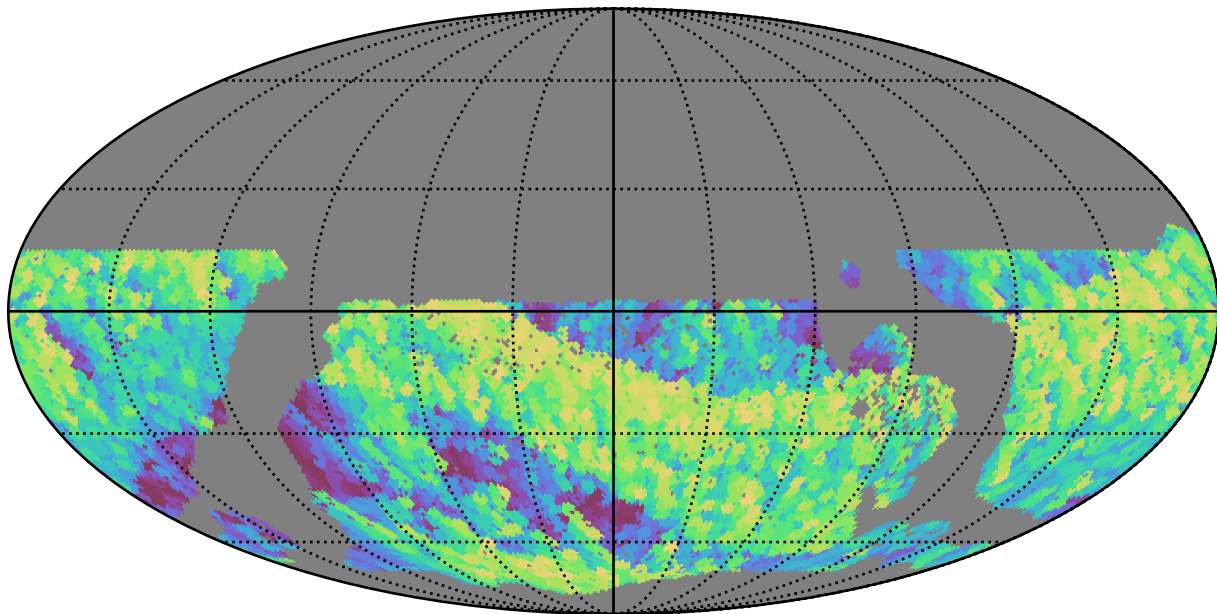
no_magell_roll_v3.4_10yrs WFD z band: Max airmass
